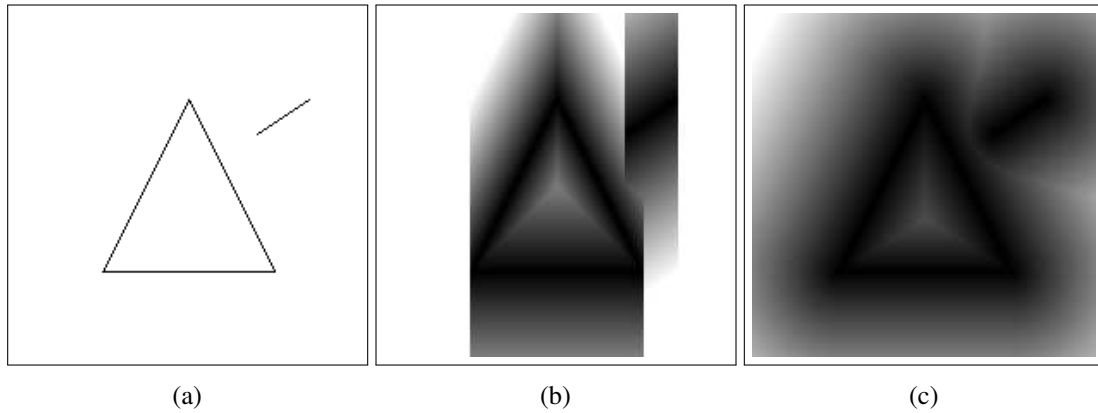
Figure 3: Illustration of the distance transform of a binary image using the squared Euclidean distance. The input image is shown in (a). The transform of the input along each column is shown in (b). The final distance transform, obtained by transforming the intermediate result along each row, is shown in (c). Dark pixels correspond to low values while bright pixels correspond to high values.
